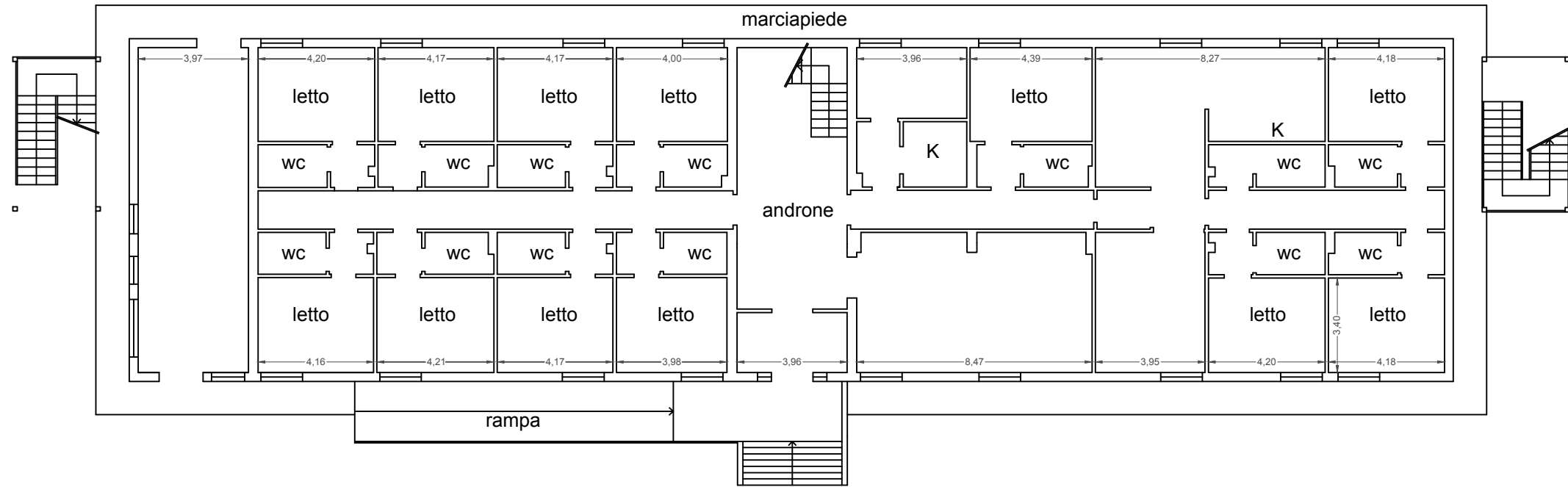
PIANO TERRA
