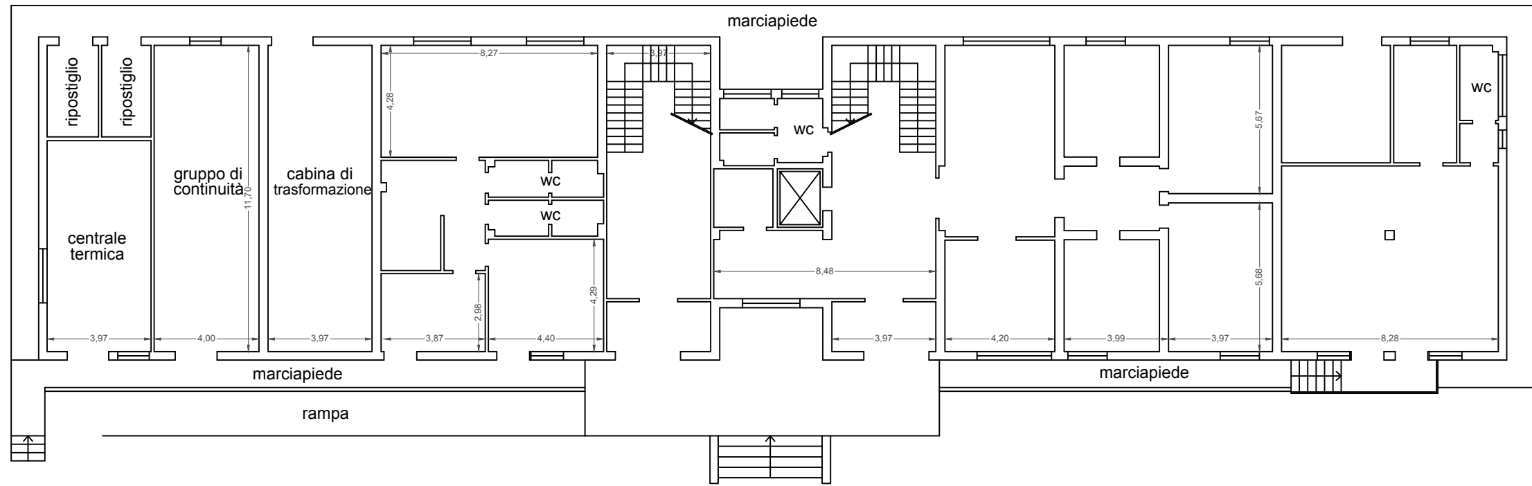
PIANO TERRA
