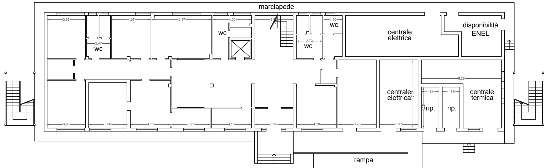
PIANO TERRA
