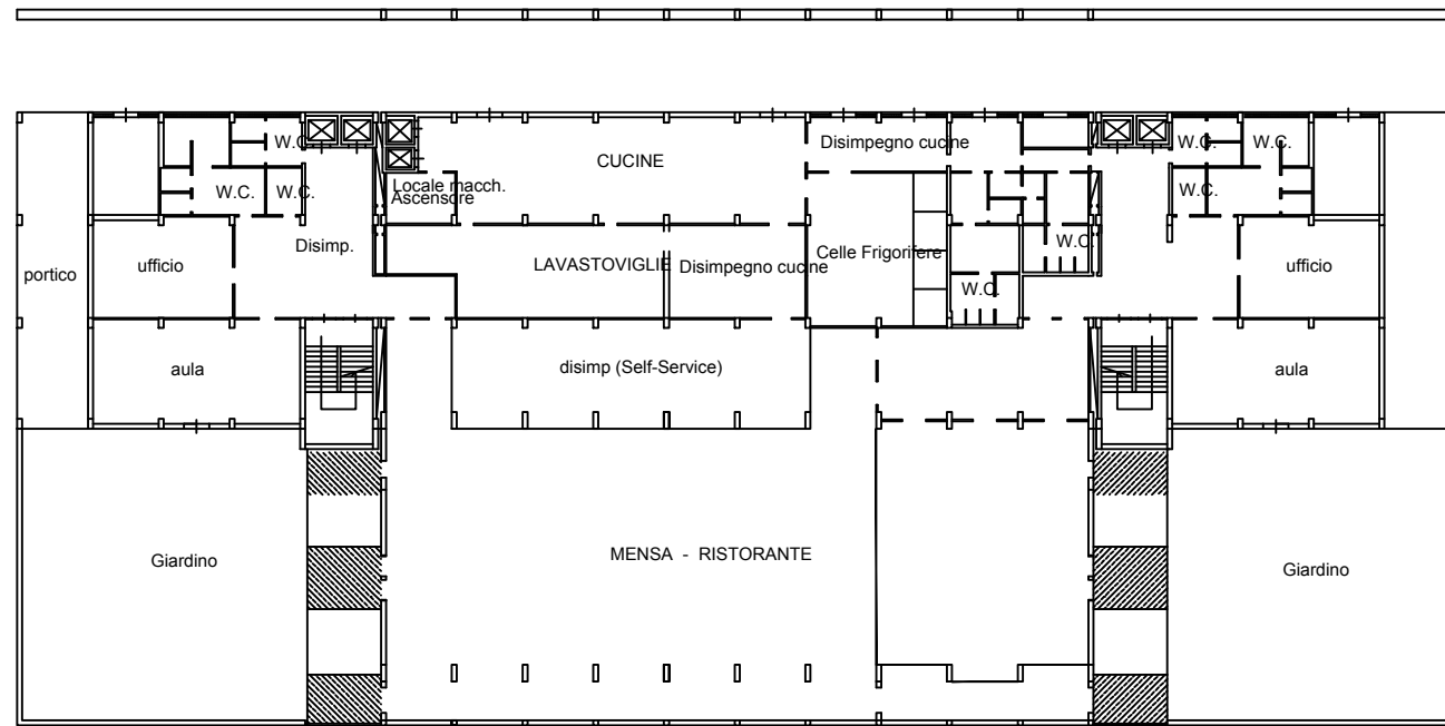
PIANO SEMINTERRATO
