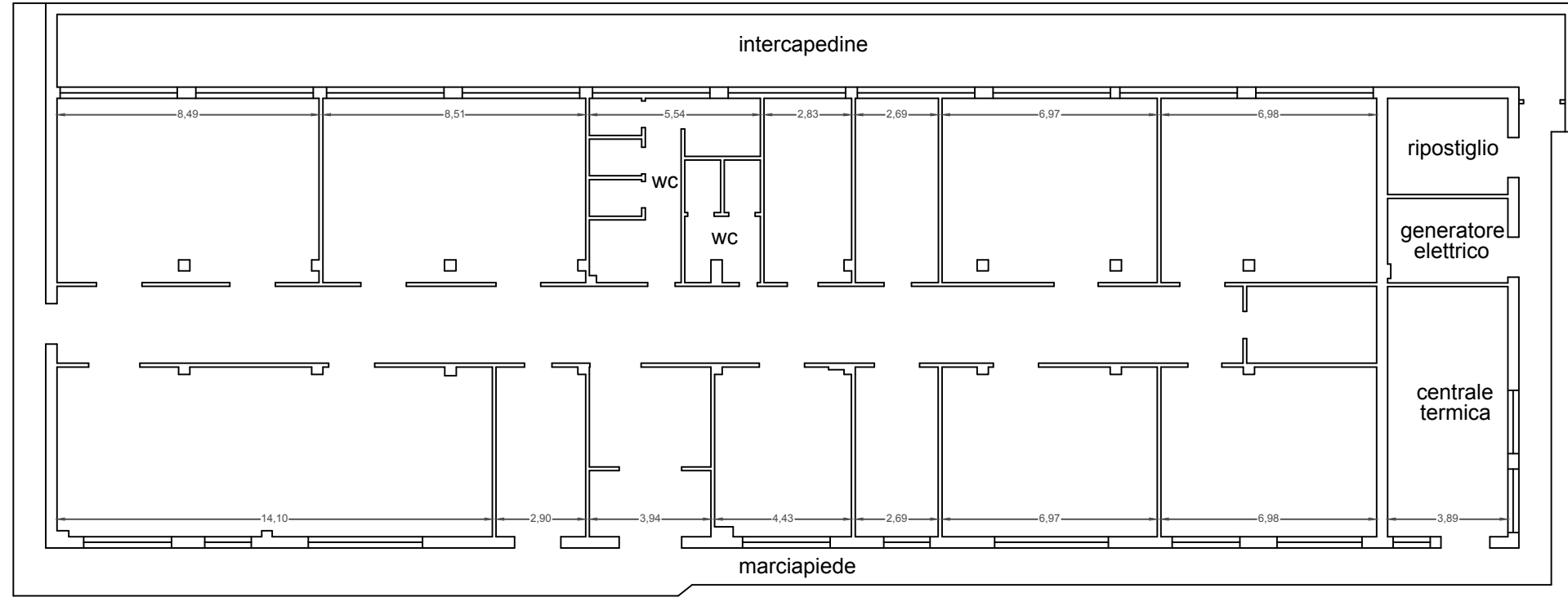
PIANO TERRA
