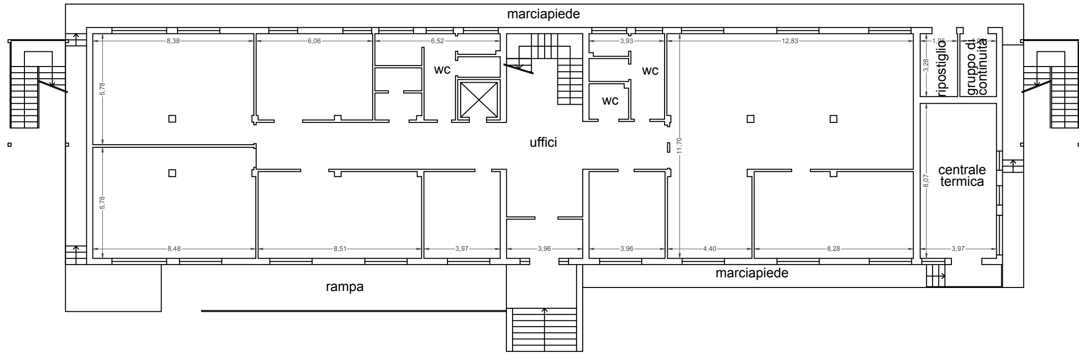
PIANO TERRA
