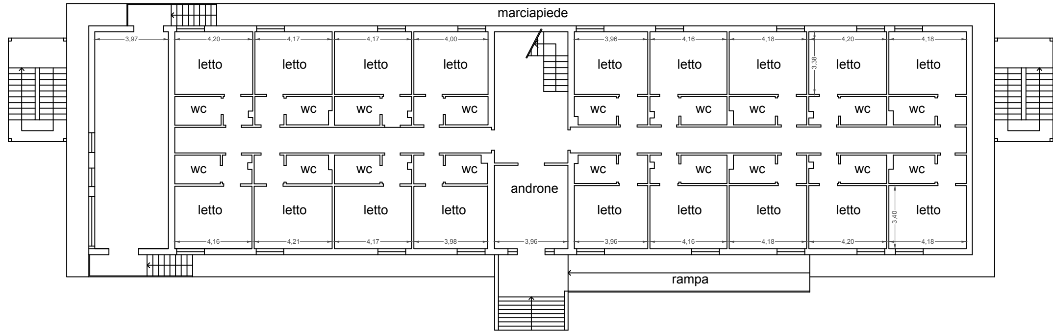
PIANO TERRA
