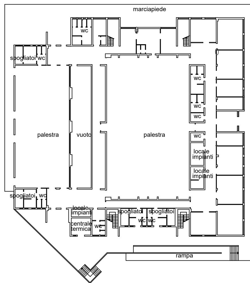
PIANO TERRA
